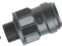
Rechte inschroefkoppeling push-in food - BSP male met O-ring
